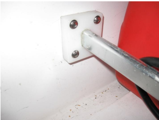
Detail of aft socket, hole in HDPVC was shaped to match profile of bar.
